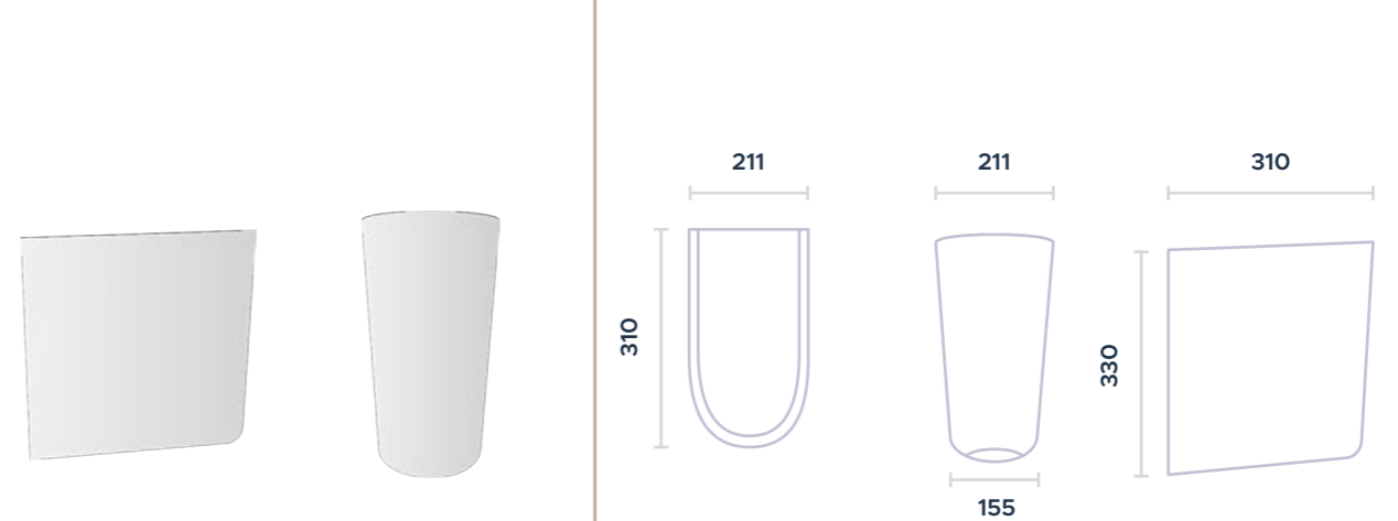
264002 ○ PEDESTAL ○ CLEAR HALF PEDESTAL
