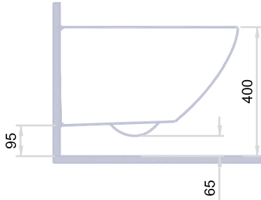
161411 WC GALIS WALL-HUNG WC PAN RIMLESS 55 CM
